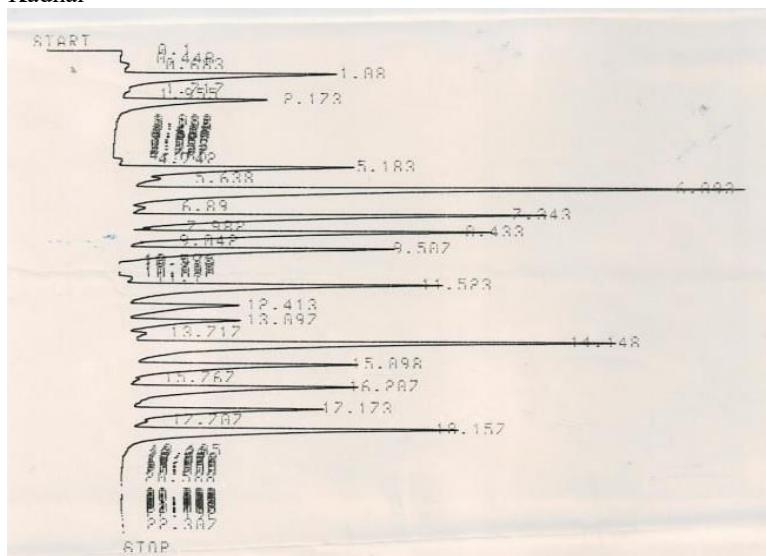
Figure 3. HPCL diagram of polyphenolic compounds of Phragmites australis collected from Rumaitha, Samawah and Kadhar.
