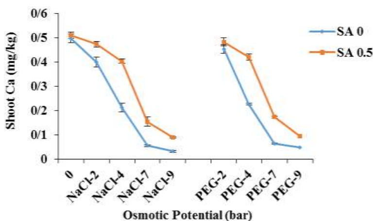
Fig. 11- Effect of different levels of salinity and drought and SA on shoot calcium content of linseed. Bars show the standard error
