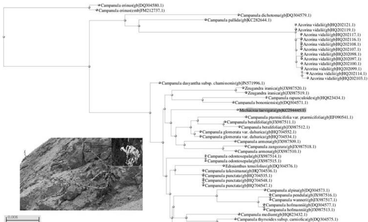
Figure 8. Phylogenetic tree of M.laevigata by the neighbor-joining method in the NCBI server; maximum sequential difference 0.1. The genus highlighted by yellow is the one detected in the present study and inscribed under the accession number KC294445.1
