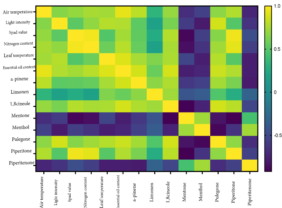
Figure 9. Correlation analysis of the studied traits under the influence of different temperature conditions (decreasing temperatures).
